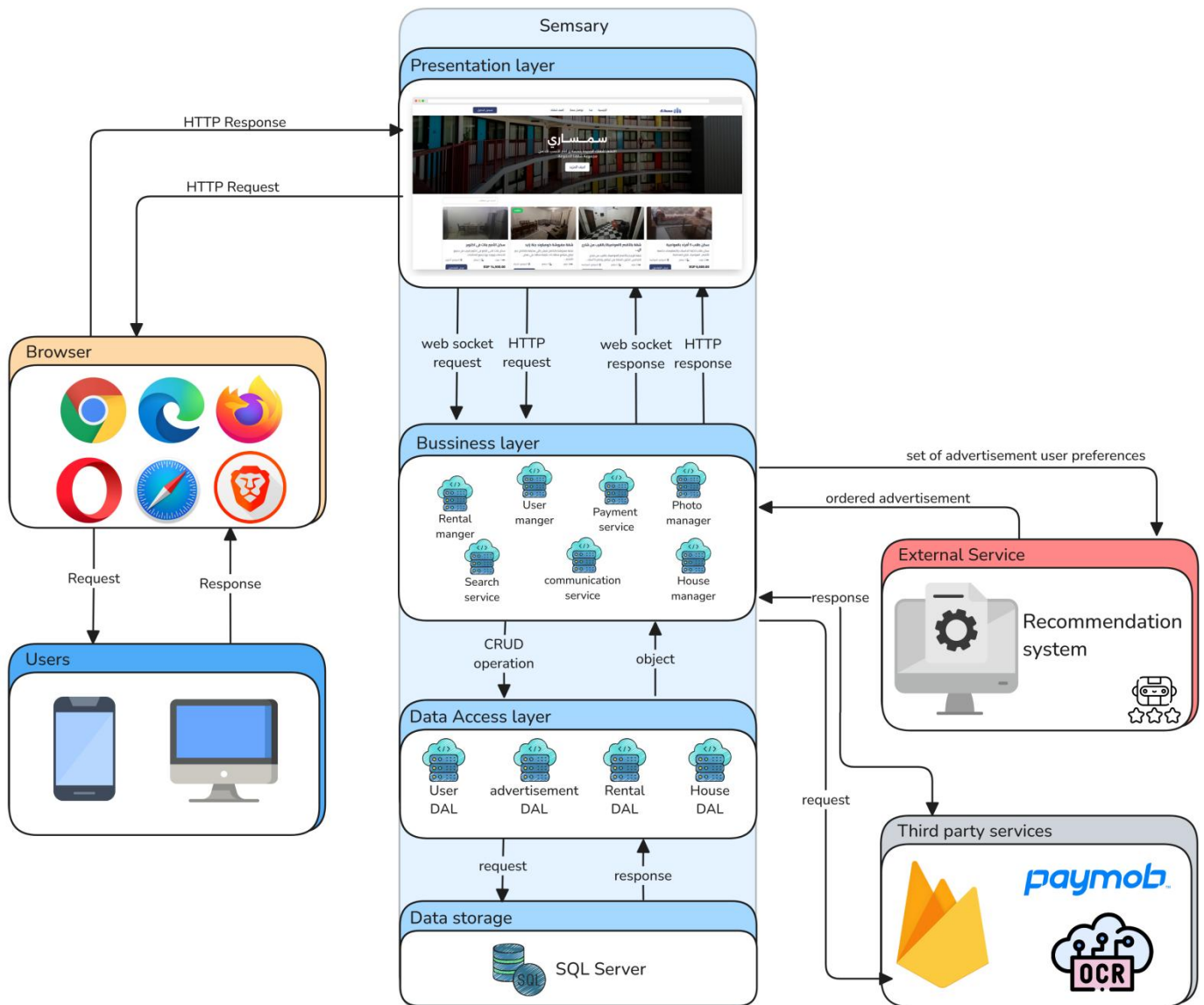
Figure 7: System Architecture diagram
