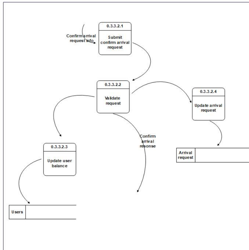
Figure 13: Data Flow Diagram 5
