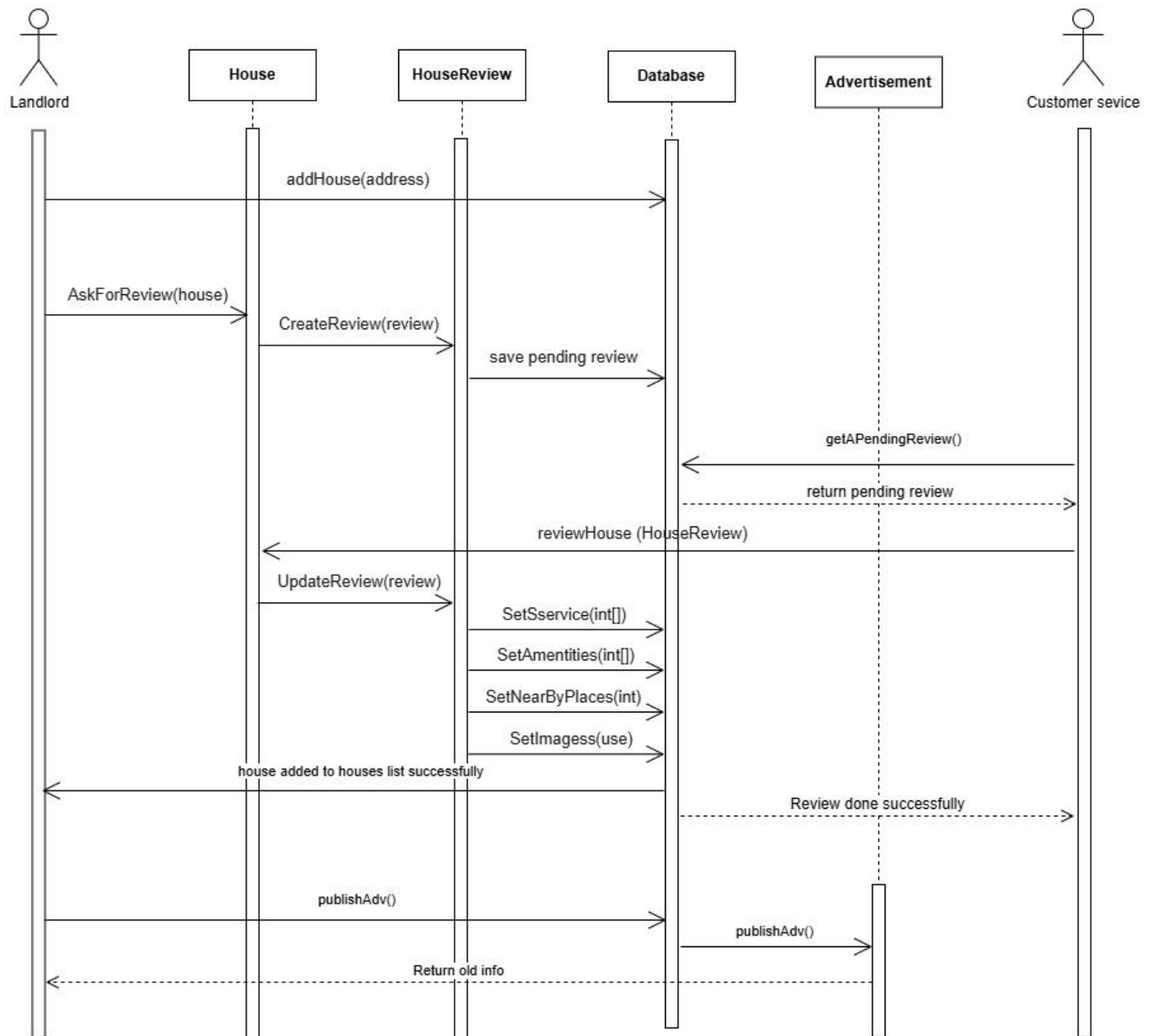
Figure 34: Sequence Diagram - Add / Publish / Review House
