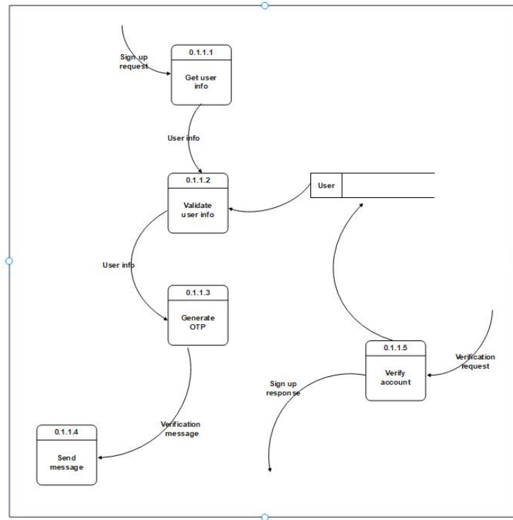
Figure 27: Data Flow Diagram 20
