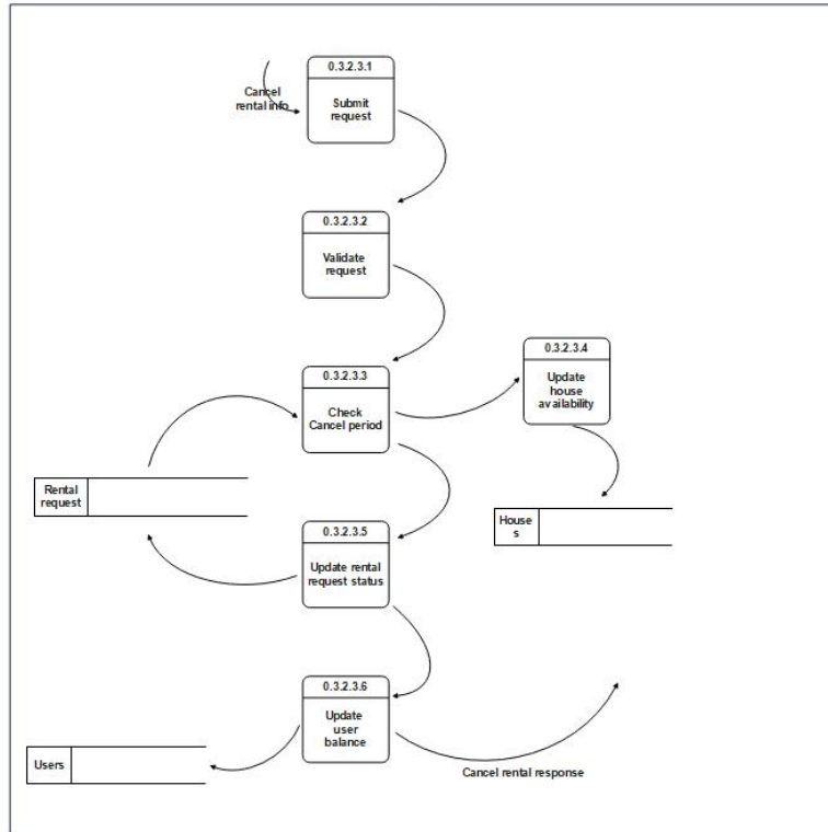
Figure 17: Data Flow Diagram 9
