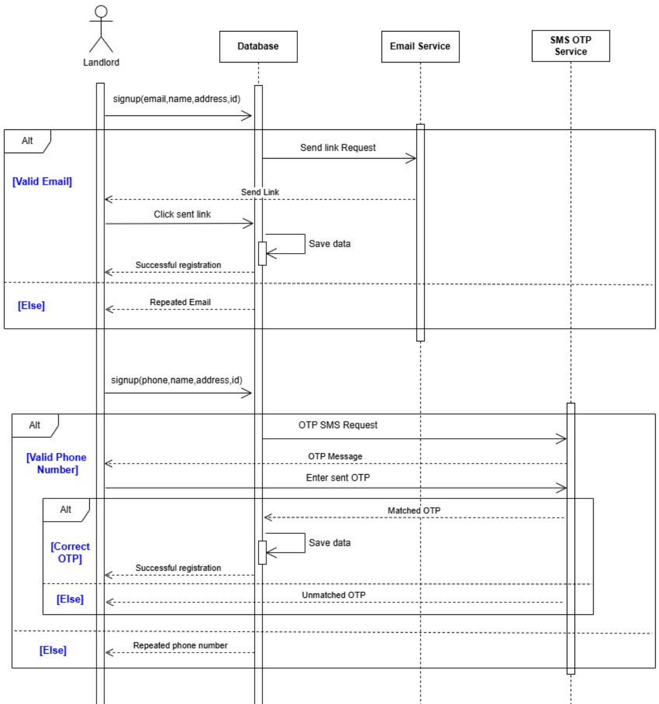
Figure 44: Sequence Diagram - Landlord SignUp
