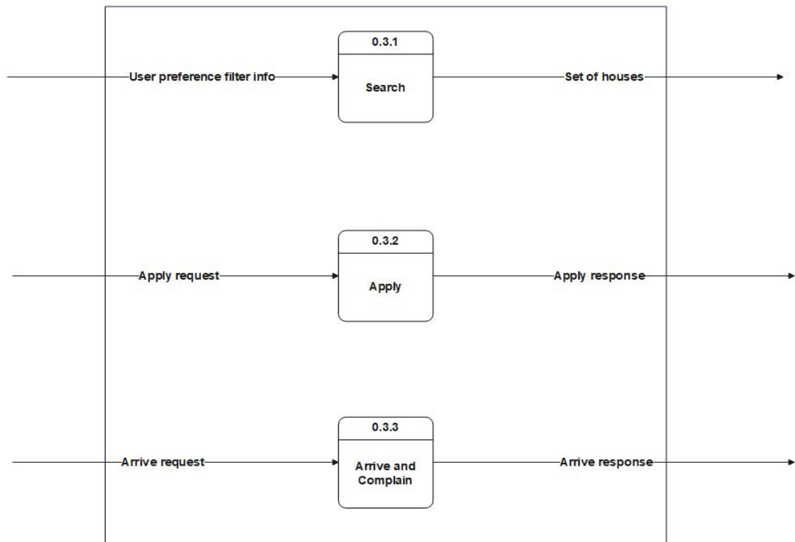
Figure 9: Data Flow Diagram 1
