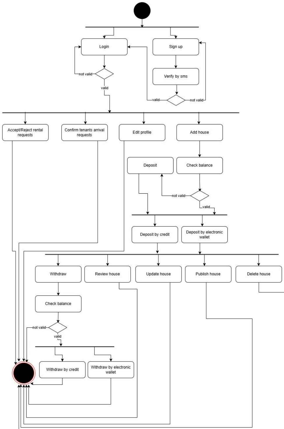
Figure 30: Activity diagrams - Landlord
