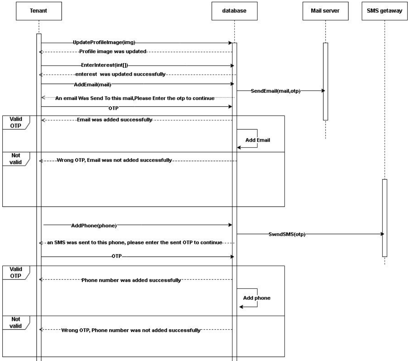
Figure 46: Sequence Diagram - Tenant Edit Profile
