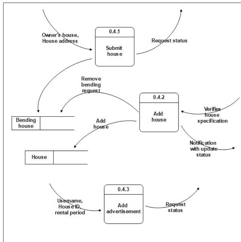
Figure 28: Data Flow Diagram 21
