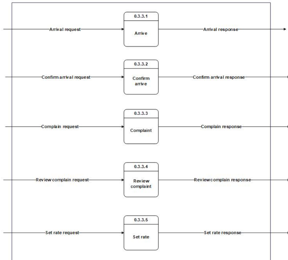
Figure 10: Data Flow Diagram 2
