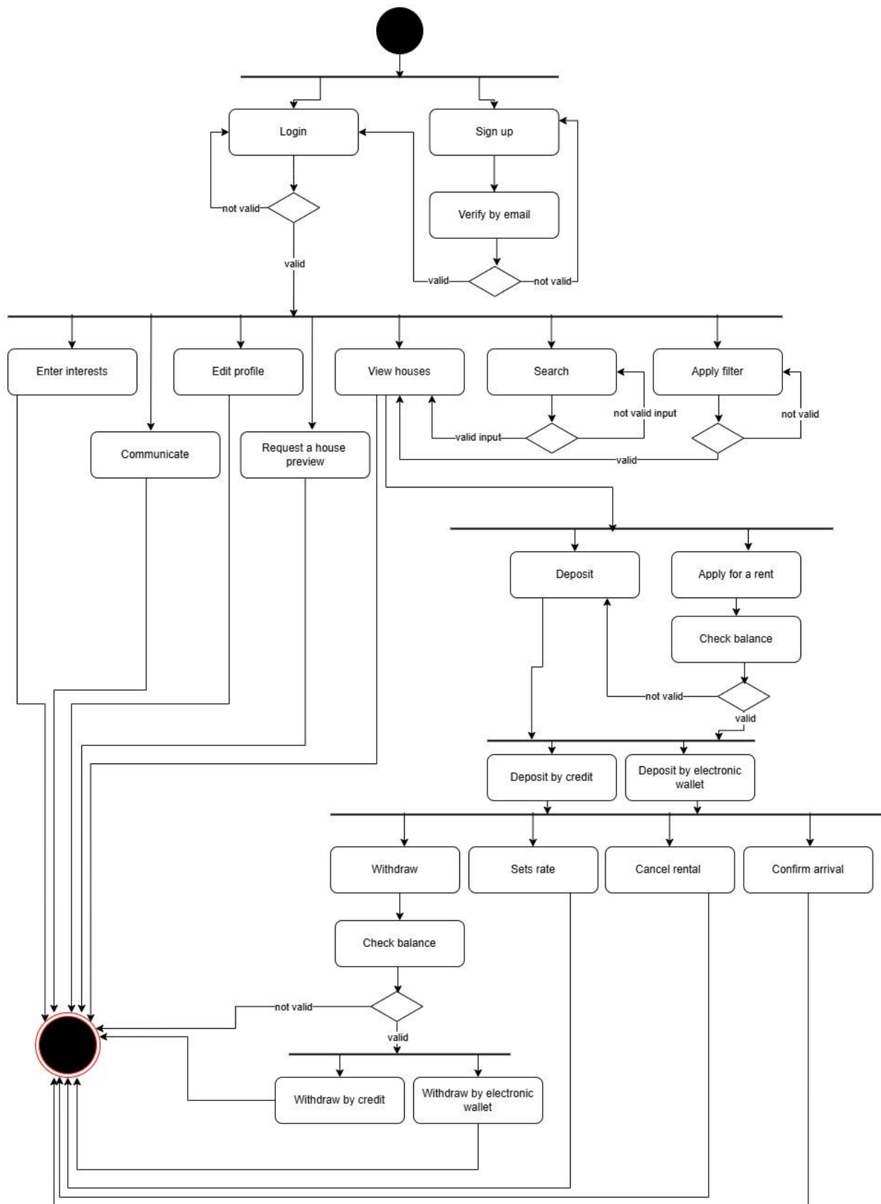
Figure 31: Activity diagrams - Tenant
